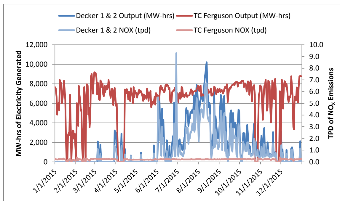
Figure 32. Comparison of Decker & T.C. Ferguson Daily Electricity Output and NO x Emissions, 2015
